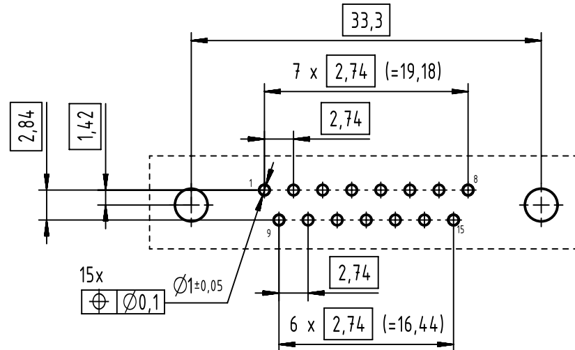
PCB layout view component side
