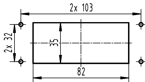
panel cut out (1:2)
