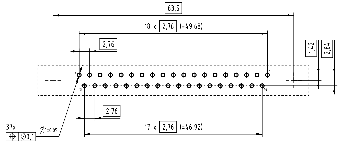
PC-Board layout view component side
