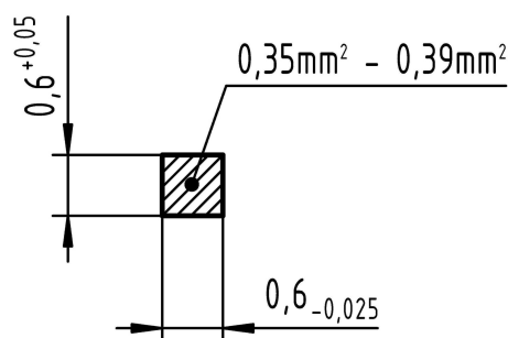
Cross section of solder termination
