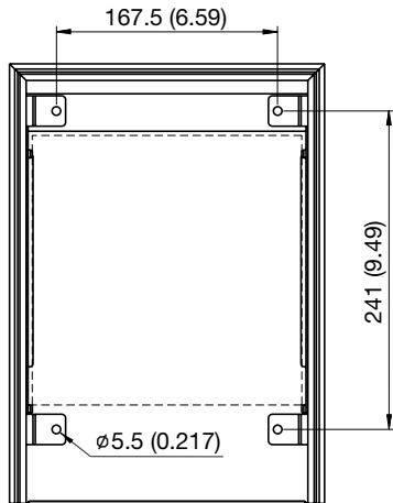
Mounting cut-out mm (in)
