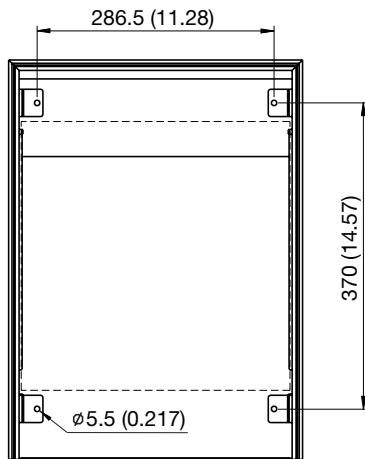
Mounting cut-out mm (in)
