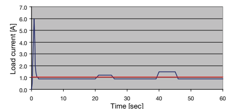
Figure 3: Ventilator
